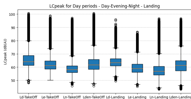
Fig. 8. Statistics of LAF and LCpeak noise levels for TakeOff and Landing aircraft activities.
