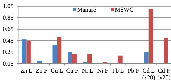
Fig. 6. Heavy metal transfer factor of cucumber tissues treated manure and MSWC (L: Leaf tissue, F: Fruit tissue).
