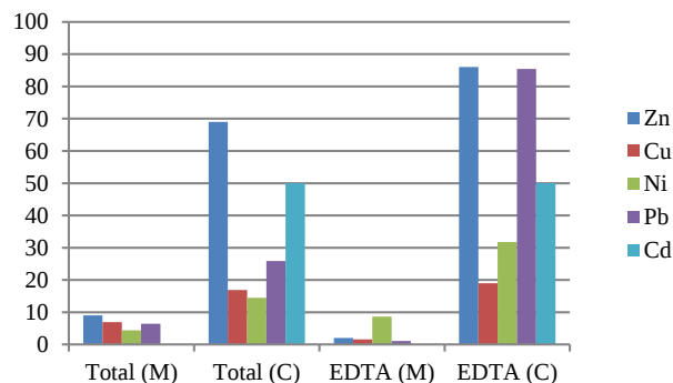
Fig. 1. Relative change of total and EDTA-extractable metal concentrations in Manure (M) and MSWC (C) applications.
