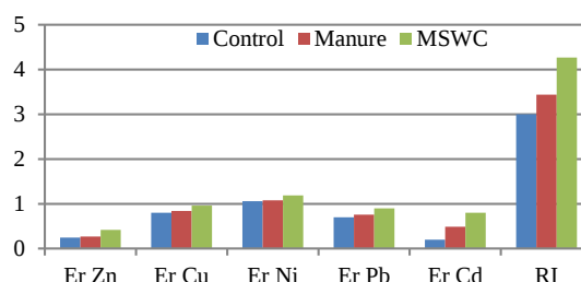
Fig. 9. Ecological risk index (Er) and Potential ecological indexes (RI) of metals in greenhouse soils treated manure and MSWC.
