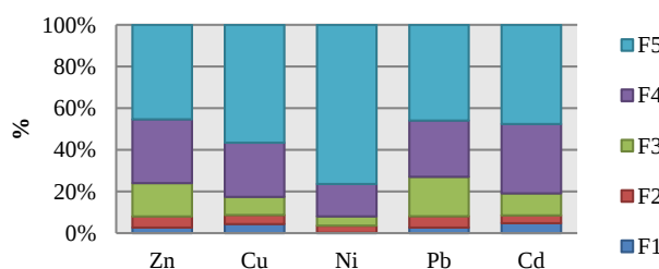
Fig. 2. Distribution of metals in the different fractions of pretreated (control) soil.
