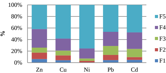
Fig. 3. Distrubution of metals in the different fractions of manure applied soil.
