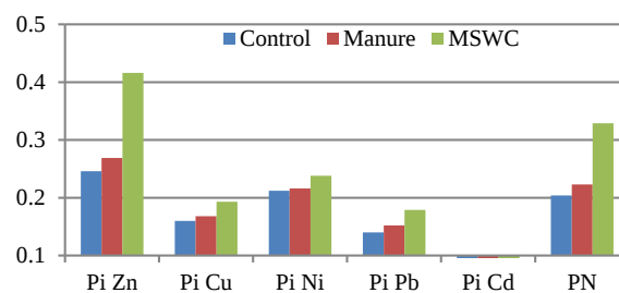
Fig. 8. Single-factor (Pi) and composite pollution coefficient (PN) of heavy metals in manure and MSWC applied soil.
