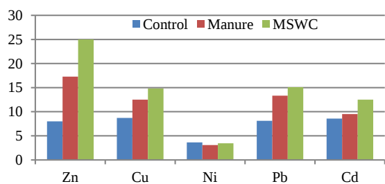
Fig. 10. RAC values of heavy metals in manure and MSWC applied soil.
