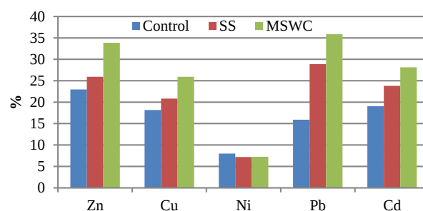
Fig. 5. Average metal mobilities of greenhouse soils treated with manure and MSWC
