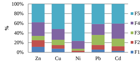
Fig. 3. Distrubution of metals in the different fractions of manure applied soil.
